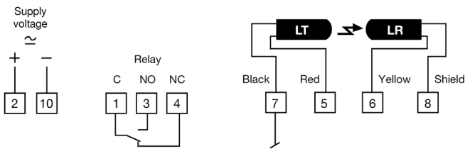
Relay output – PA 10 A/B 51X
